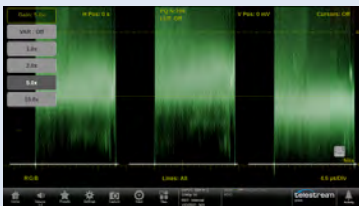
Gain adjustment for fine adjustment of black or white levels.
