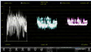
YPbPr waveform display to isolate difference between luma and color components. Color trace can be selected in application menu.
